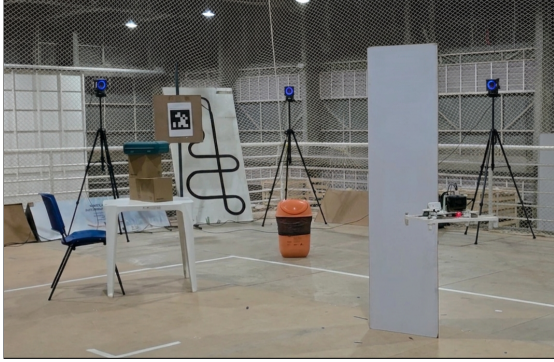
Figure 3: Experimental Setup. (a) Controlled indoor flight volume for the open-vocabulary object-goal trials, with the quadrotor, marked operating bounds, and everyday referents. (b) Cluttered setup for the path-planning trials (Sec. 4.3), with a table, chair, tool case, and a freestanding vertical panel placed between the take-off pose and the trash-bin referent.
